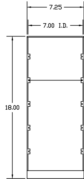
TRAY DETAIL
