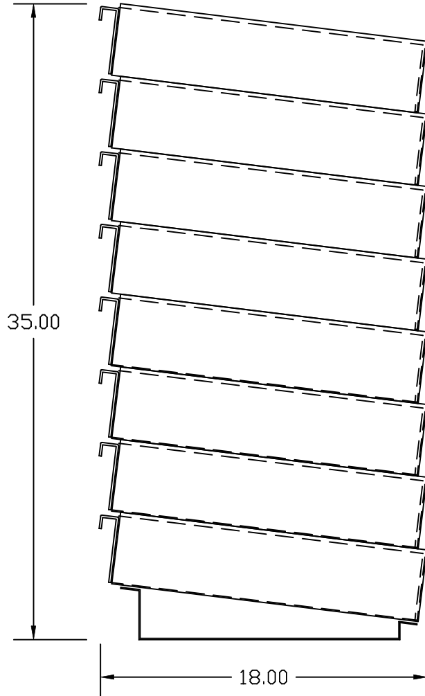
SIDE VIEW
