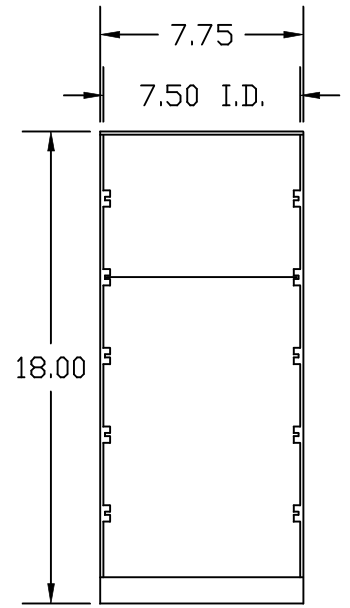
TRAY DETAIL
